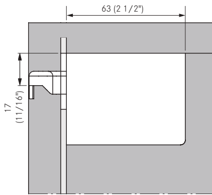
Fixture for cabinet
